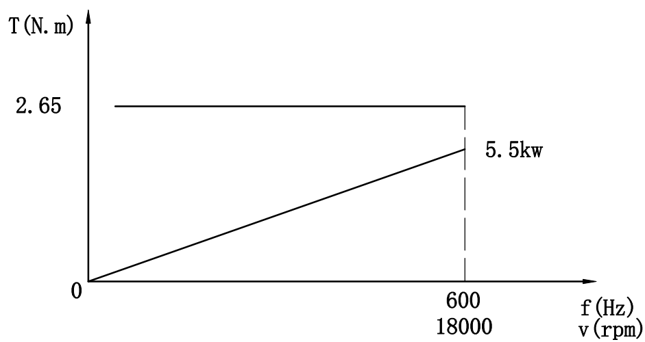
扭矩/功率曲线 Torque/P. f Curve
