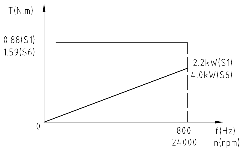
Torque/P.f Curve
