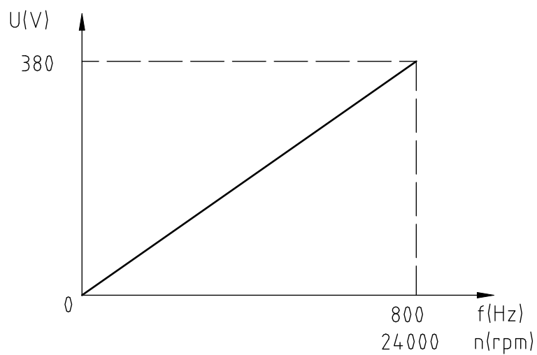
U.f Curve
